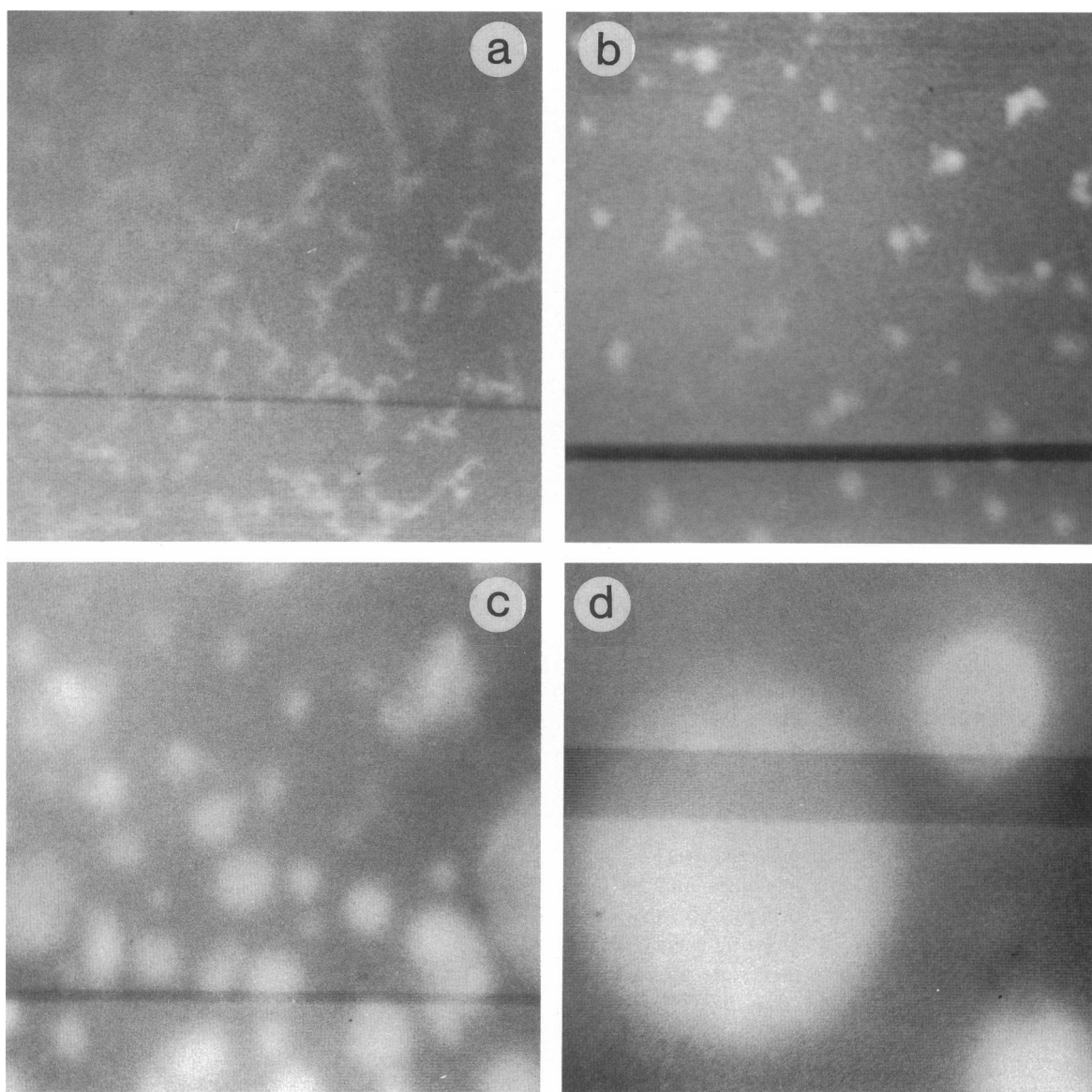
FIGURE 3 Fluorescence photomicrographs of FTSVs adhering to decane-based BLMs. FTSVs adhere to BLMs, forming aggregates. Lenses form under the aggregate (a) and, over the course of several minutes, the lenses coalesce (b–d). Decane-based PS-PE BLMs were painted and allowed to thin in MbK. MbK containing 15 mM \text{CaCl}_2 and 10 \mu\text{M} \text{CoCl}_2 was perfused into the upper chamber. FTSVs were then added and allowed to settle onto the BLM, after which unbound FTSVs and external calcein were removed by perfusion with MbK containing 15 mM \text{CaCl}_2 and 10 \mu\text{M} \text{CoCl}_2 . The width of each photograph corresponds to 47 \mu\text{m} . The pictures were recorded with a silicon-intensified target video camera. Single frames from videotape were photographed.
