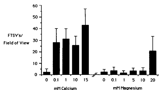
FIGURE 6 Binding of FTSVs to BLM depends upon the concentration of \text{CaCl}_2 and \text{MgCl}_2 . BLMs were spread and allowed to thin in MbK and solutions containing calcium or magnesium chloride were perfused into the upper chamber. FTSVs were then added and allowed to settle down onto the BLM. The number of FTSVs bound per field of view was counted under epi-fluorescence illumination using a 100 \times water immersion lens. Bars represent the mean number of FTSVs per field of view and the lines represent one standard deviation. The field of view was 85 \mu\text{m} in diam.
